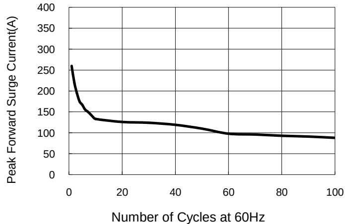
Fig 4. Non-repetitive Forward Surge Current
