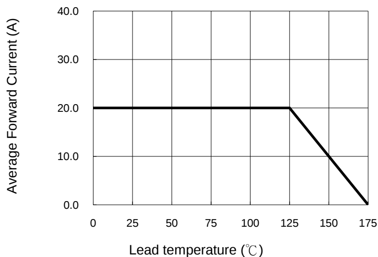
Fig 3. Typical Forward Current Derating Curve
