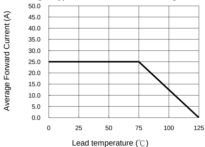
Fig 3. Typical Forward Current Derating Curve
