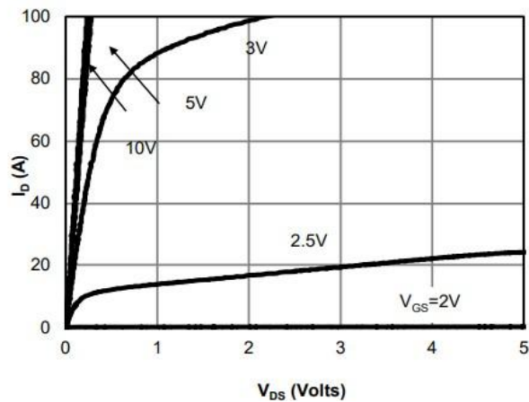
On-Region Characteristics
