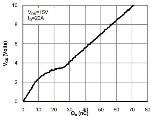
Gate-Charge Characteristics
