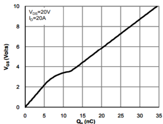
Gate-Charge Characteristics
