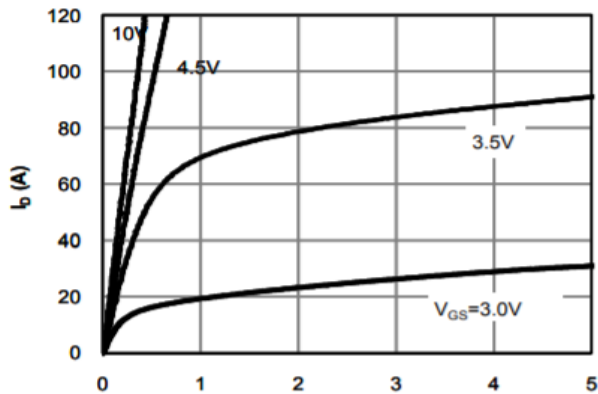
On-Region Characteristics
