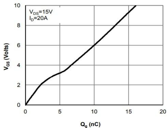
Gate-Charge Characteristics
