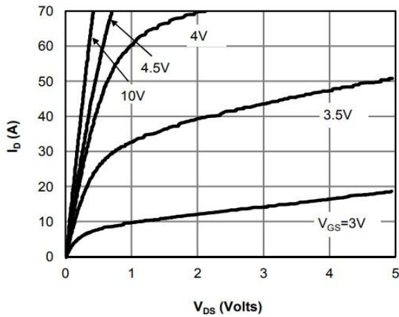
On-Region Characteristics
