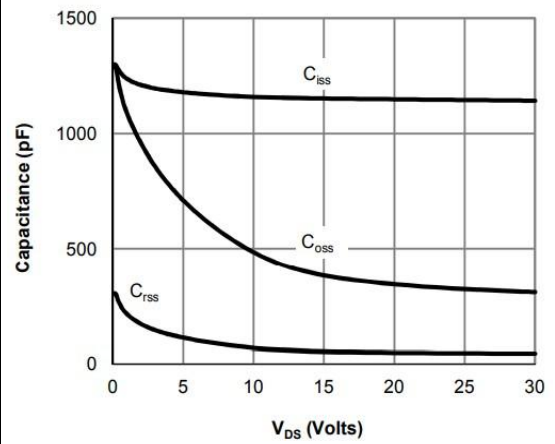
Capacitance Characteristics
