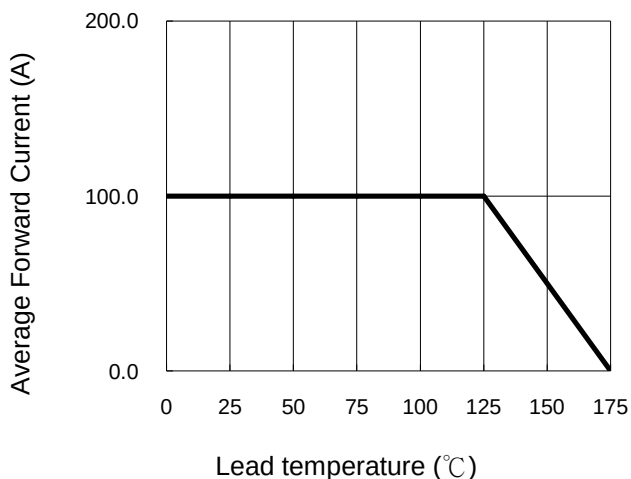
Fig 3. Typical Forward Current Derating Curve
