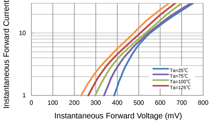
Fig 1. Typical Forward Characteristics
